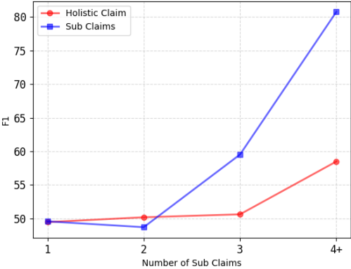
Fine-Grained vs Holistic Verification (Llama-3.1 Generated Sub Claims)
